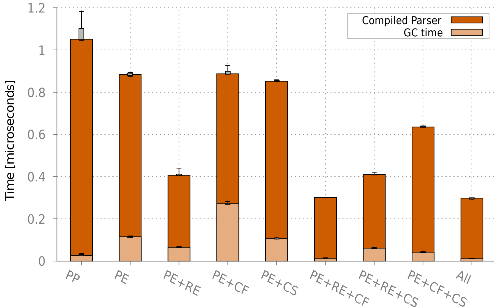
Time per Character of Smalltalk
