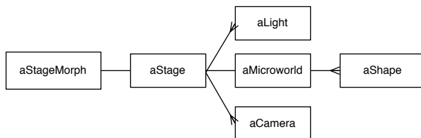
Figure 4. Lumiere Stage Model Entity Diagram
