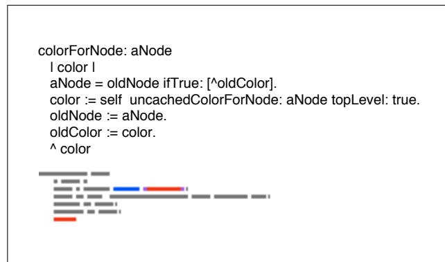
Fig. 5. The control flow microprint of the method colorForNode: reveals it contains a guard clause.
