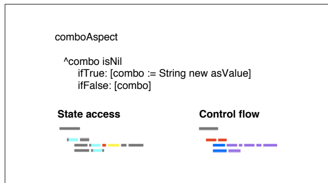
Fig. 4. Microprints of an accessor method following the lazy initialization pattern
