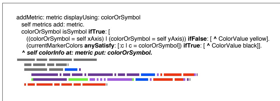
Fig. 6. A complex control flow microprint.
